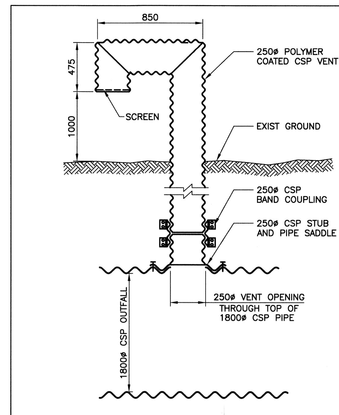
250Ø CSP VENT DETAIL SCALE: NTS
