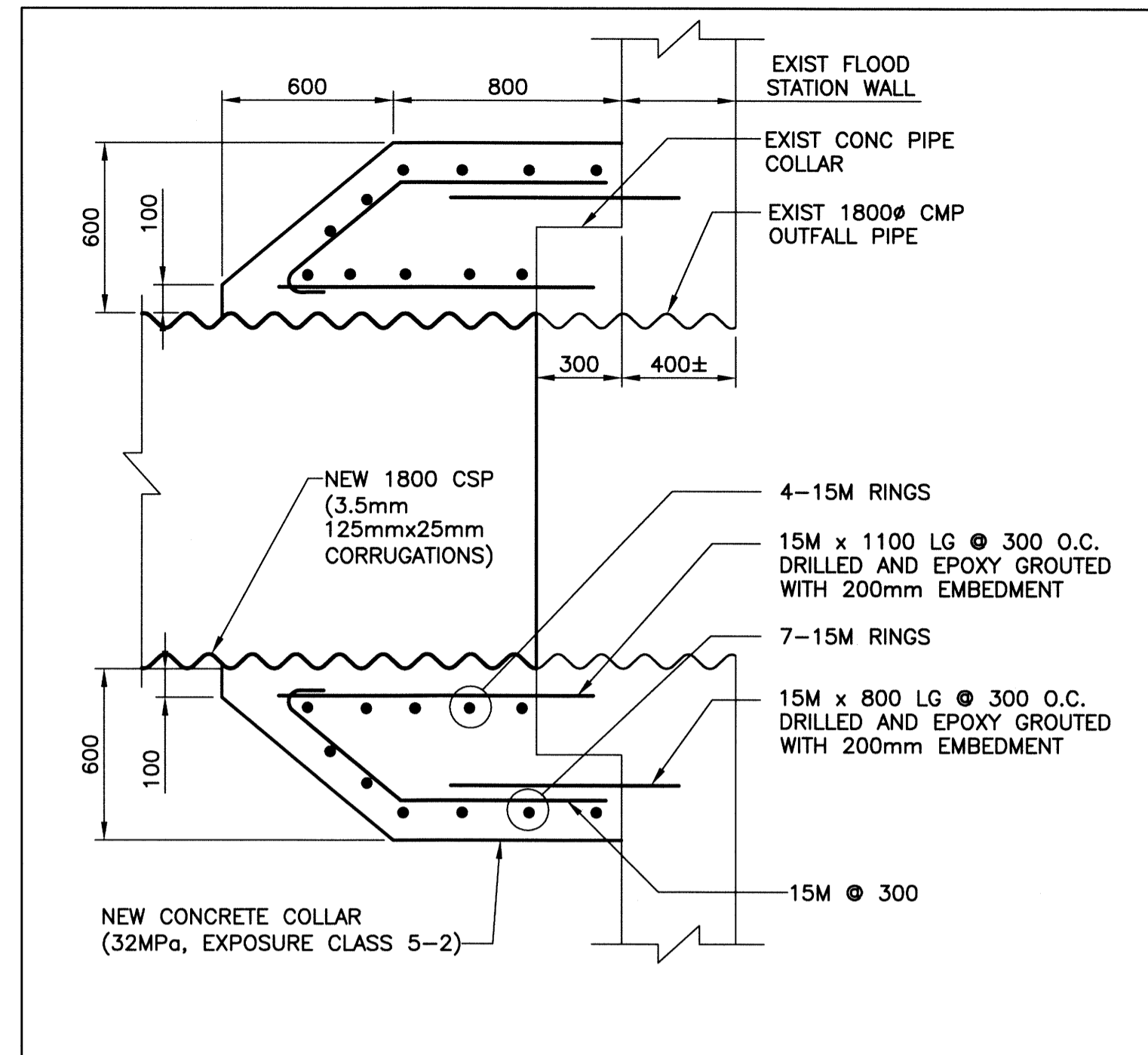
REINFORCED CONCRETE COLLAR DETAIL SCALE: NTS
